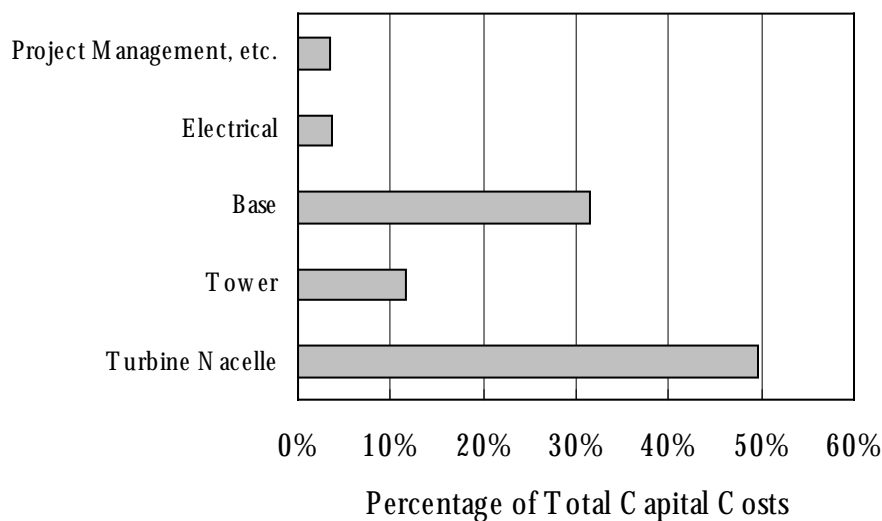
Figure 4.3 Breakdown of Capital Costs of an Offshore Wind Turbine
