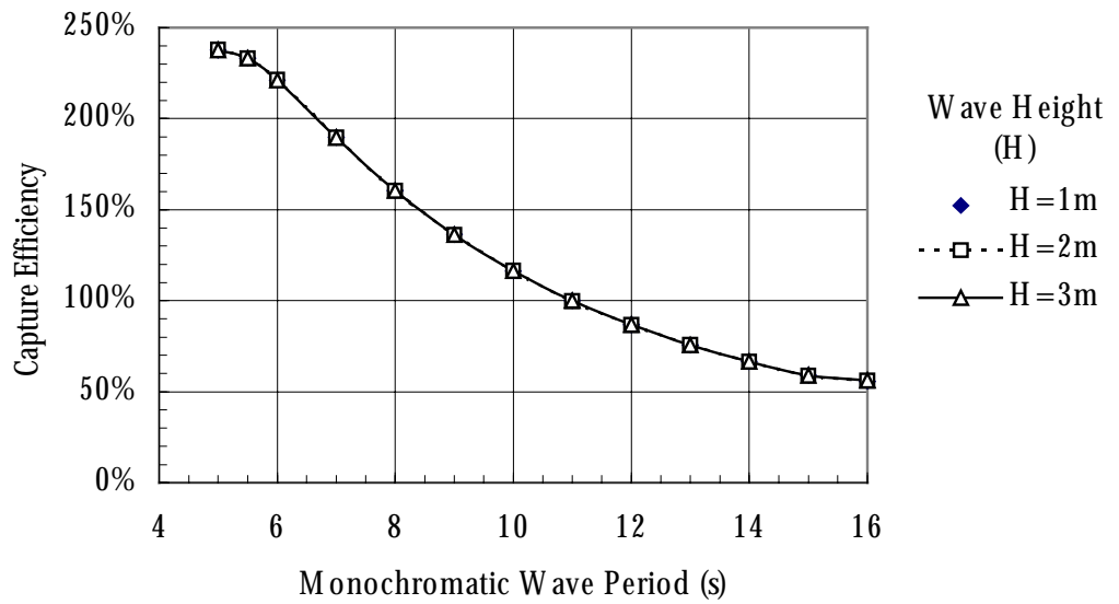
Figure 6.11 Predicted Capture Efficiency of an MWP in Real Seas
