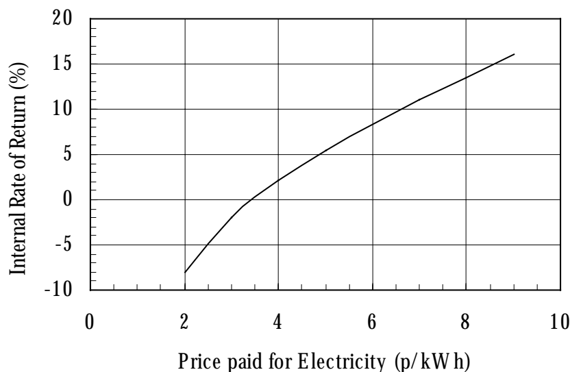
Figure 6.14 Internal Rate of Return on an MWP Scheme
