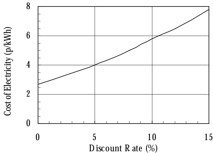
Figure 4.9 Influence of Discount Rate on the OSPREY's Generating Costs
