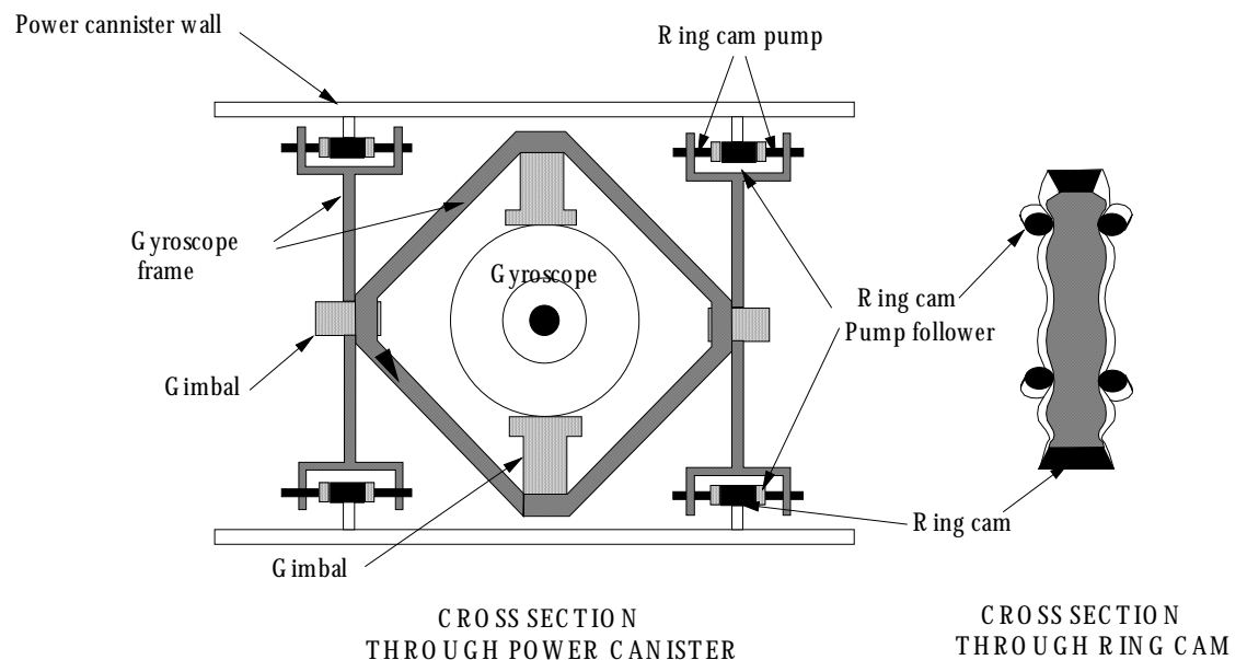
Figure 5.3 Schematic of the Gyroscope and Ring Cam Pump Assembly
