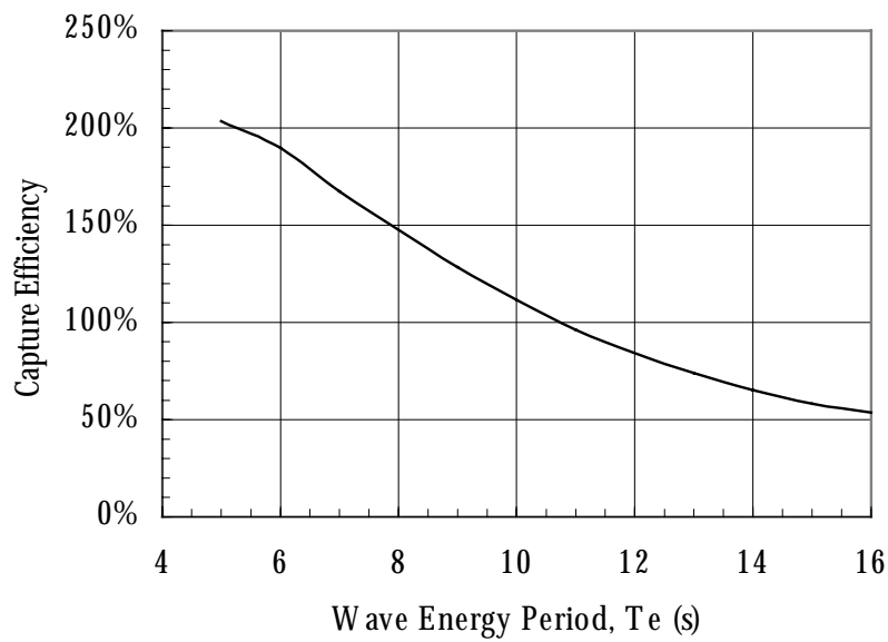
Figure 6.11 Predicted Capture Efficiency of an MWP in Real Seas
