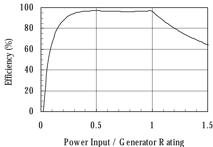
Figure 4.7 Operating Characteristics of the Generators
