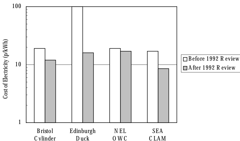
Figure 9.3 Change in Predicted Electricity Costs in 1992 Review
