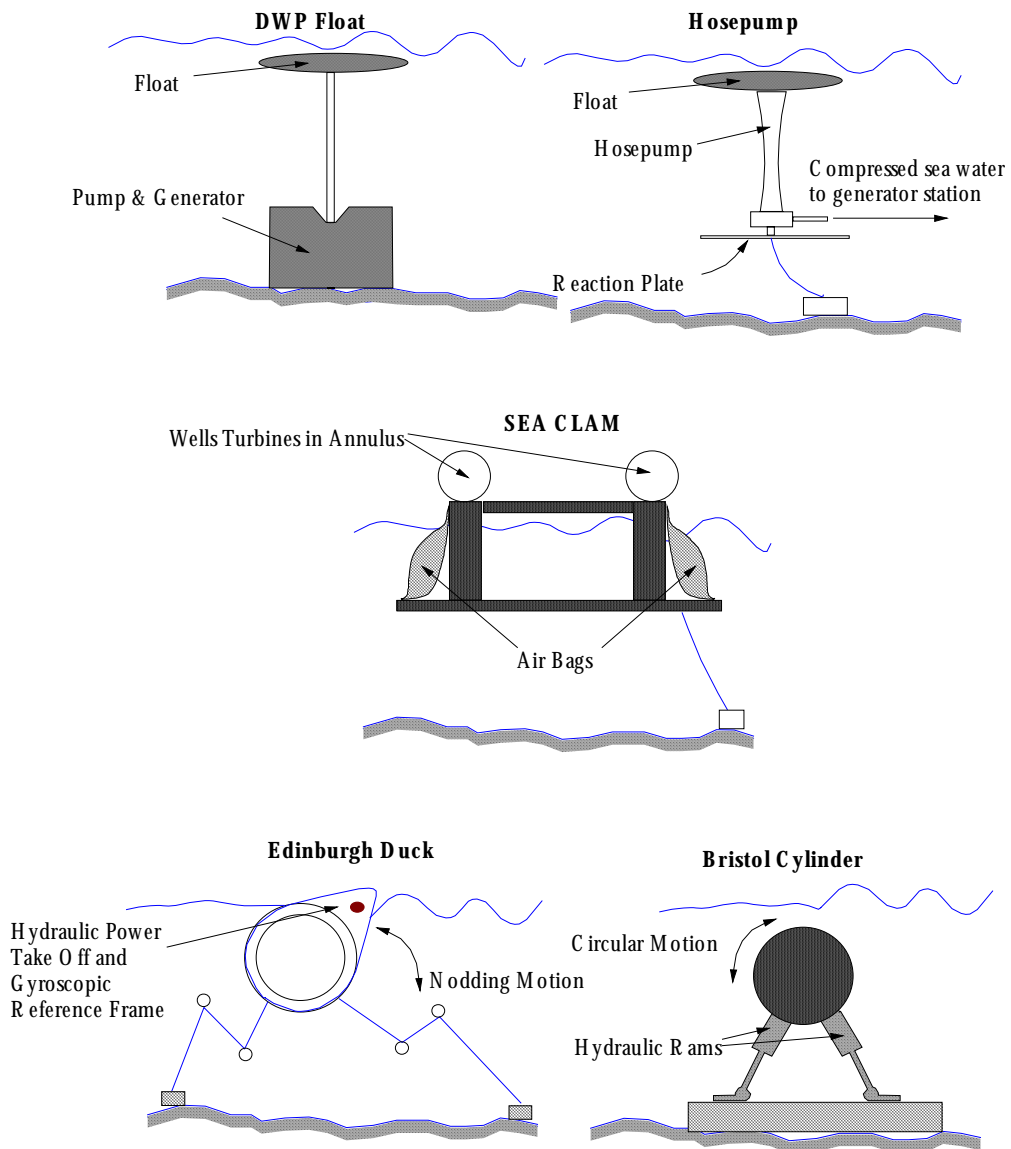
Figure 7.2 Offshore Wave Energy Devices
