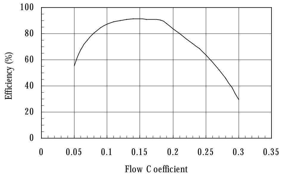
Figure 4.6 Operating Characteristics of the OSPREY Wells' Turbine
