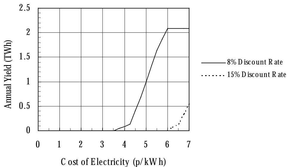
Figure 4.11 Cost-Resource Curves for Existing OSPREY
