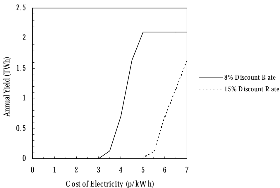
Figure 9.6 UK Nearshore/Shoreline Wave Energy Resource Cost Curves*
