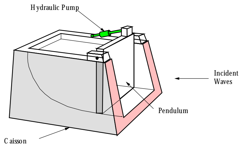
Fig. 7.1c Pendulum Device
