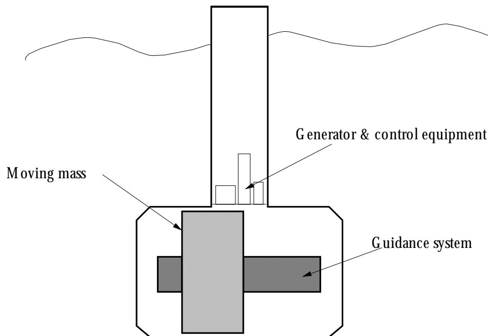
Schematic View
