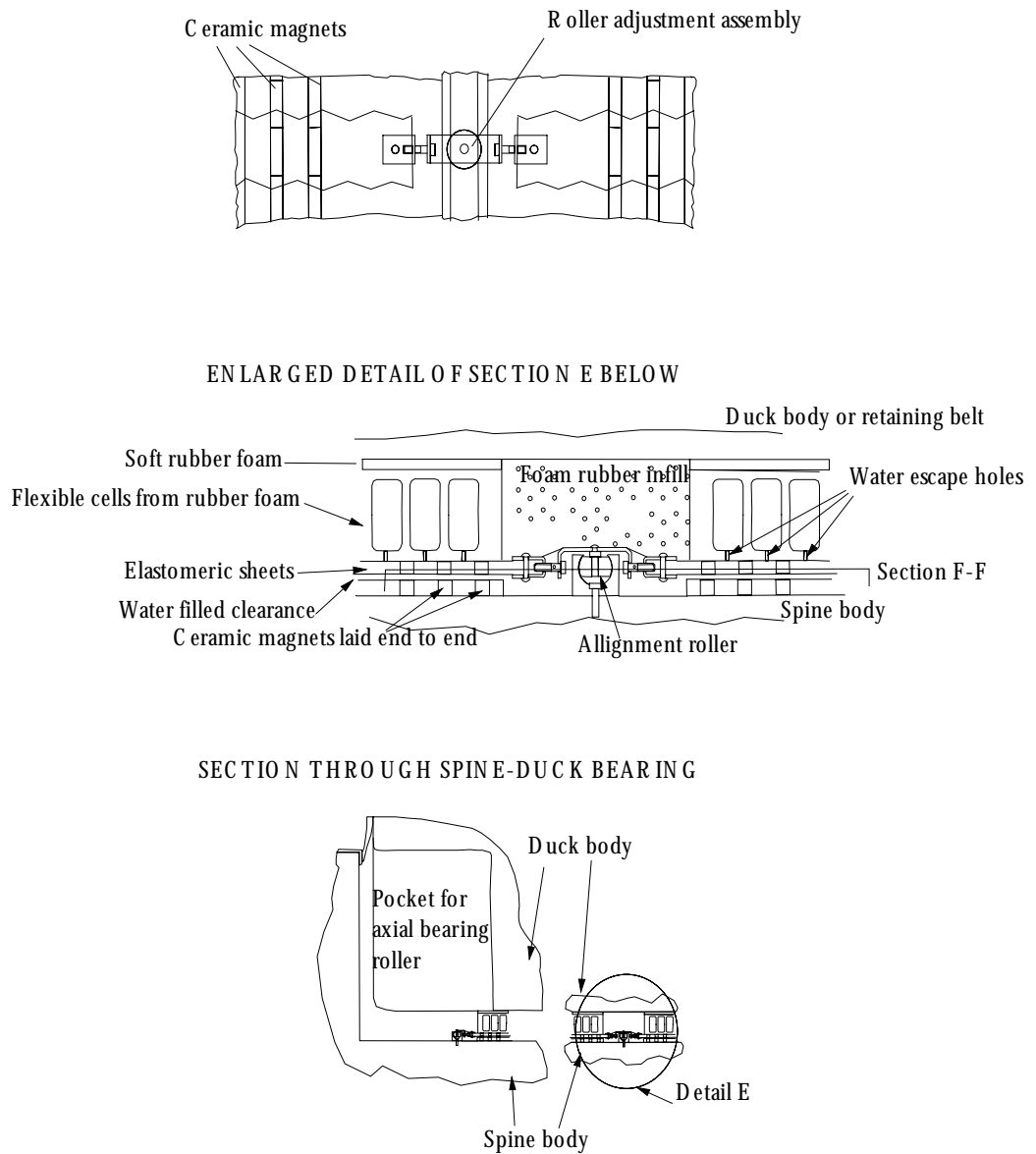
Figure 5.10 The Duck-Spine Slubber Bearing RADIAL VIEW OF SPINE-DUCK BEARING
