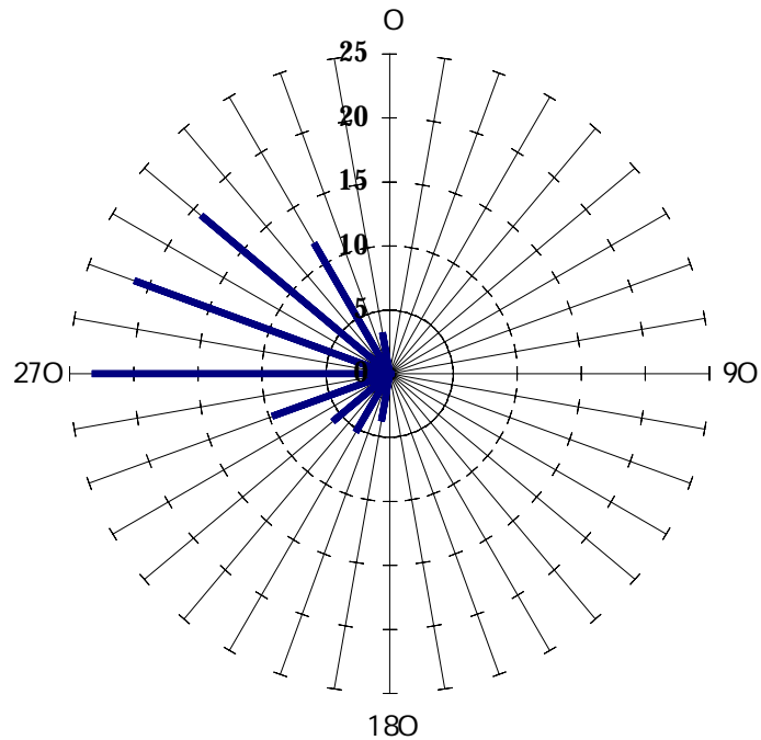
Figure 2.2 Wave Rose for 100 m Water Depth West of UK*
