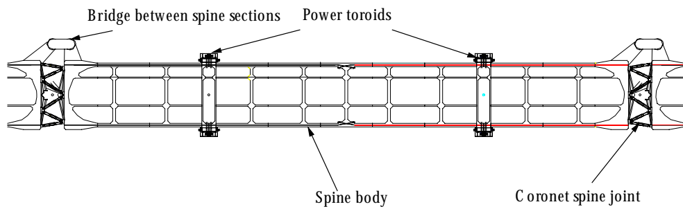
Figure 5.6 New Spine Design and Hinged Bridges for the 1998 Duck
