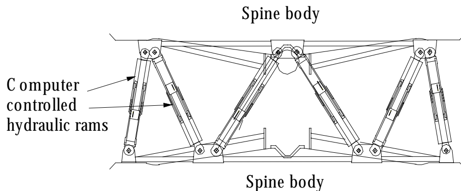
Figure 5.9 The Coronet Assembly for Connecting Spine Sections
