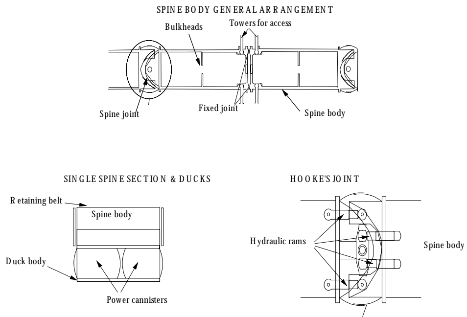
Figure 5.2 Main Features of the Duck-Spine Assembly
