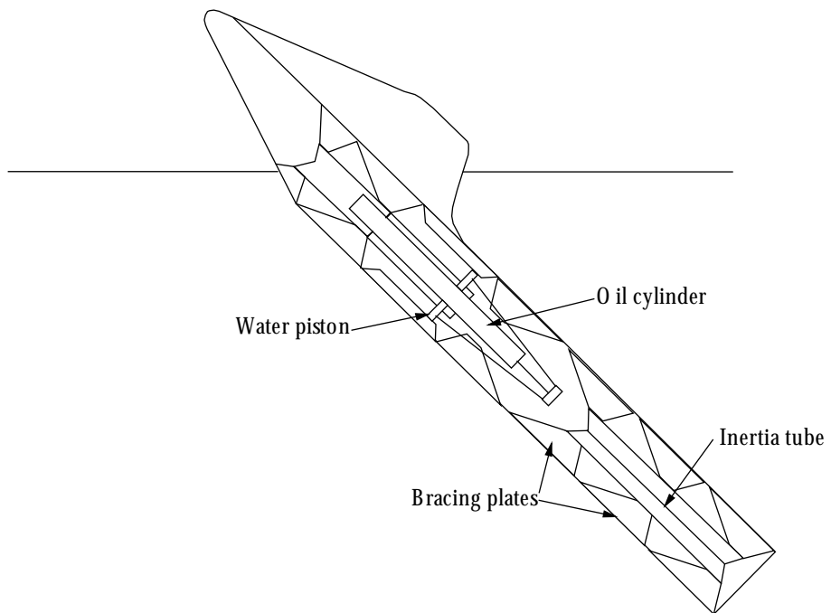
Figure 6.16 Side View of the Sloped IPS Buoy
