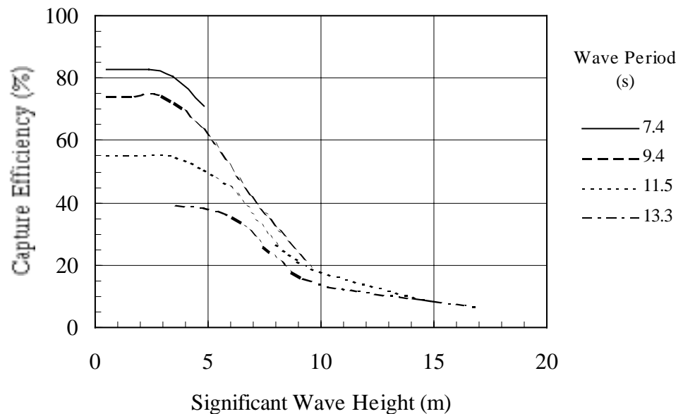
Figure 5.12 Capture Efficiency of the Duck
