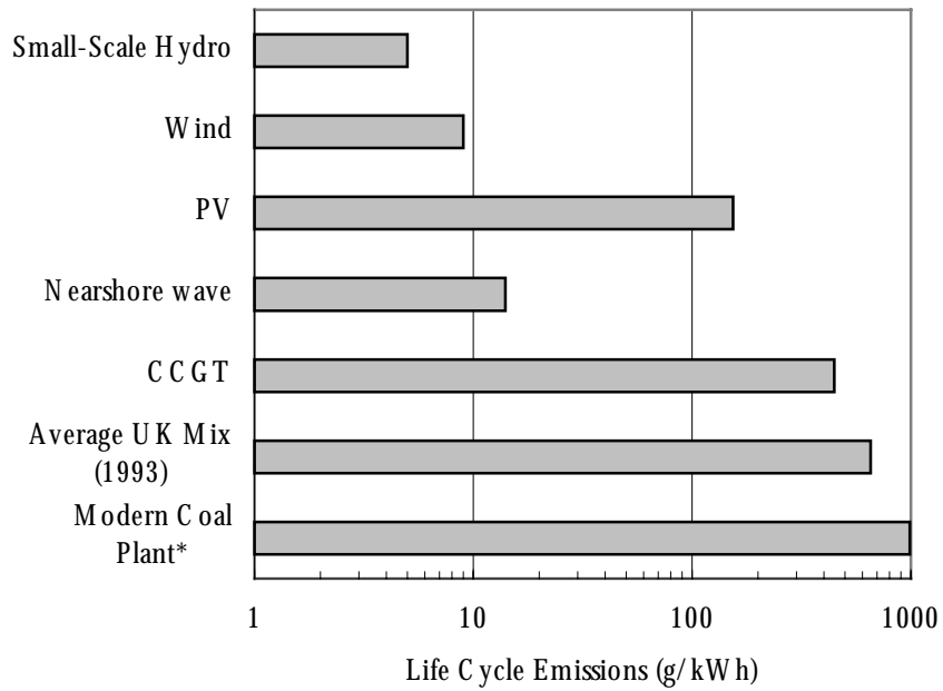
Figure 8.1 Comparison of Life Cycle Emissions of CO 2
