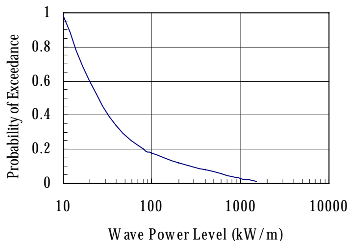
Figure 2.3 Representative Distribution of Wave Power Levels
