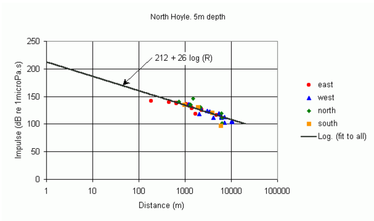
Figure 31. The measured impulse of pile hammering noise in dB re 1 \mu Pa.s at North Hoyle at 5 m depth, and impulse Source Level and Transmission Loss best fit.
