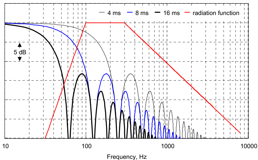
Fig. 3-3. Spectra of rectangular impulses of different lengths and assumed radiation function of the pile
