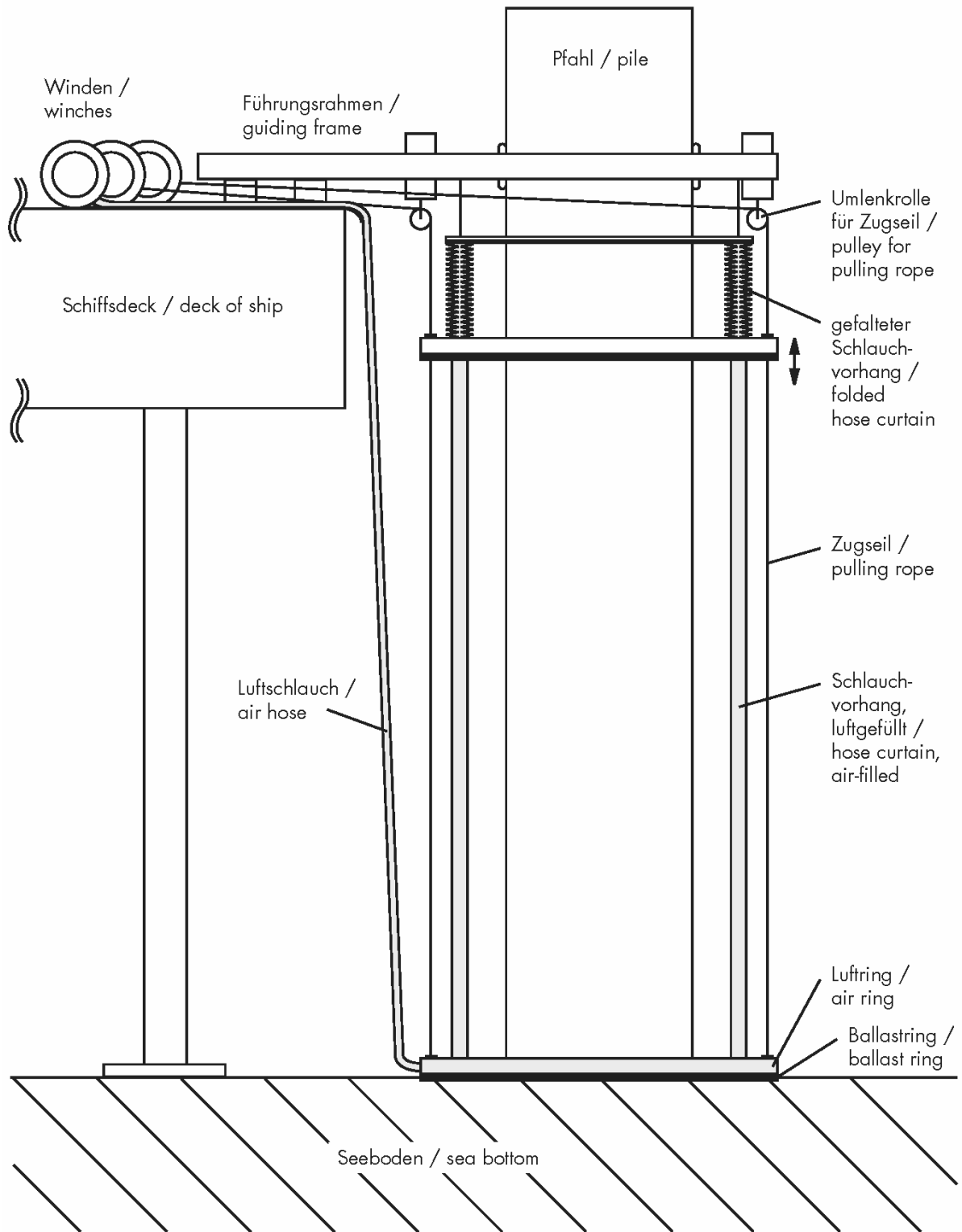
Figure 3-30. Inflatable noise mitigation system; side view
