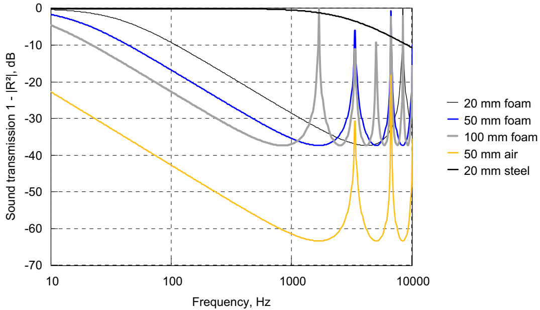
Figure 3-22. Sound level reduction obtained with layers containing air, computed after equation 3.6 and 3.5. Incidence angle = 0^\circ , foam density = 30 \text{ kg/m}^3 . Steel, for comparison, is a poor sound insulator for water-borne sound.
