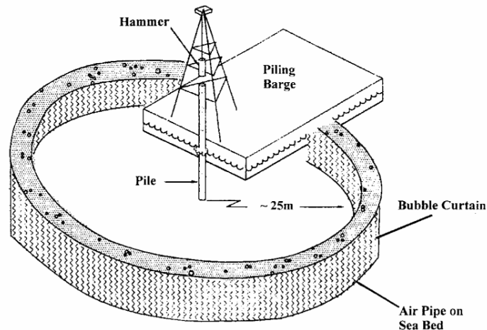
Fig. 3-13. Bubble curtain setup by Würsig et al. (2000)
