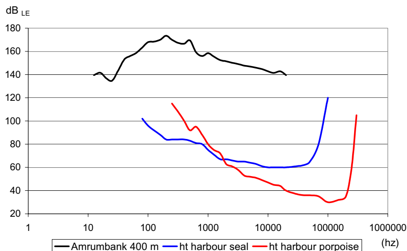
Fig. 2.8. Hearing thresholds of harbour porpoise and harbour seal and noise from underwater pile driving. Sources: Noise emissions (SEL) from pile driving at Amrumbank (North Sea, Germany) (ISD et al. 2007). Hearing thresholds: lower values from data compiled by Thomsen et al. (2006).
