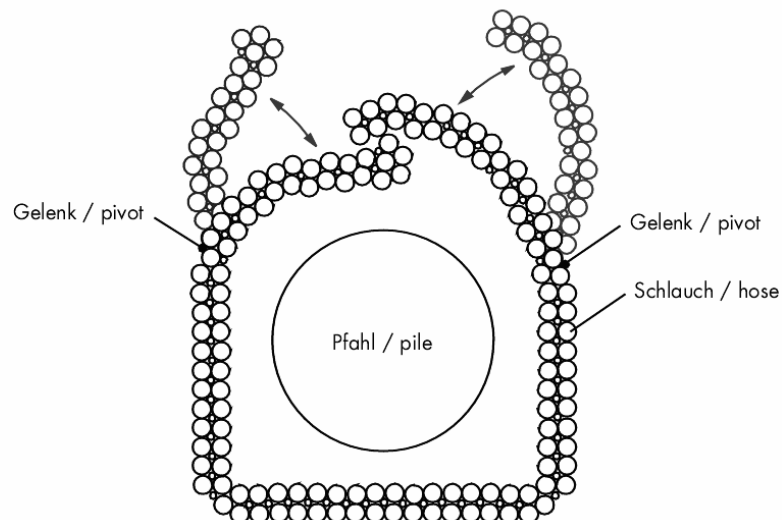
Figure 3-33. Top view of hose curtain
