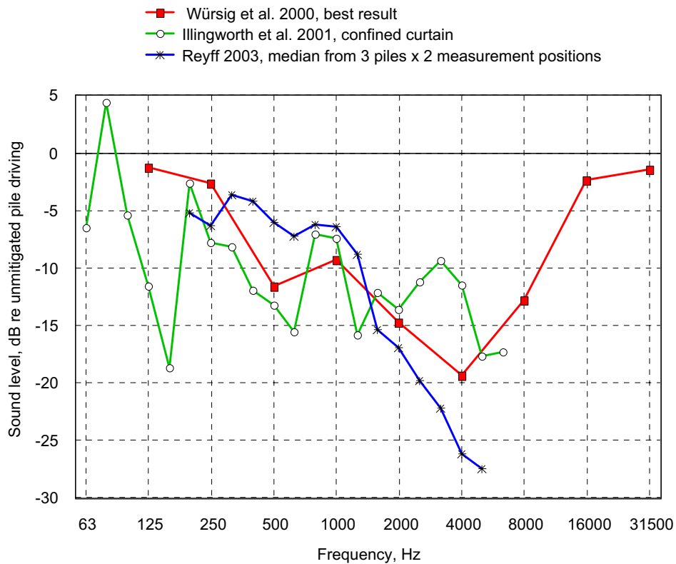
Fig. 3-18. Sound attenuation versus frequency for some of the bubble curtains in Table 3.1
