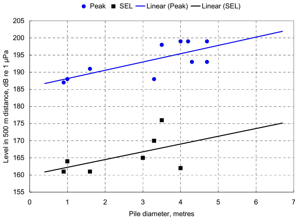
Fig. 2-7. Peak and SEL levels from Table 2.1 as a function of pile diameter
