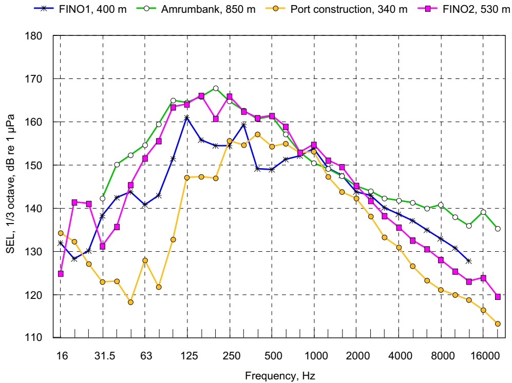
Fig. 2-3. Spectra for some of the of pile driving operations listed in Table 2-1
