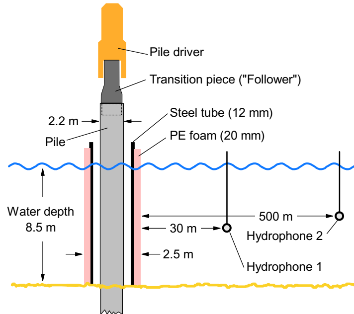
Figure 3-24. Setup for evaluating a pile sleeve (Schultz-von Glahn et al. 2006)
