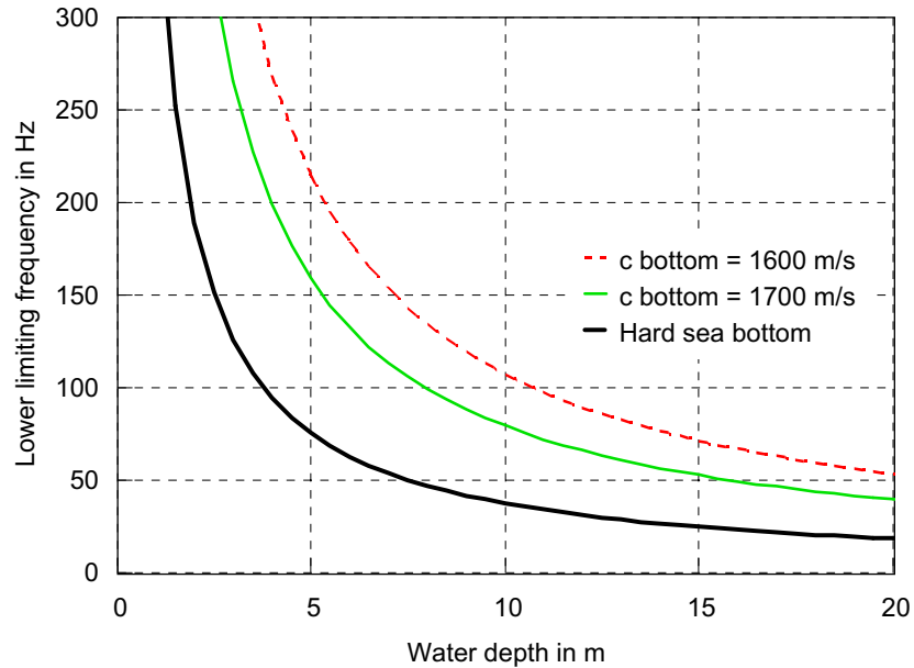
Fig. 2-4. Lower limiting frequency of propagation as a function of water depth, after equation 2.8. Sound below this frequency is attenuated much stronger than the maximum geometric transmission loss 20 \log(R) .
