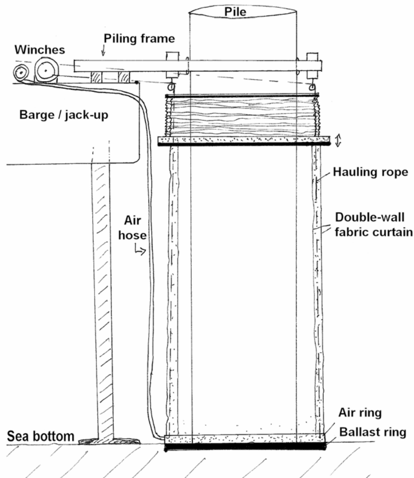
Fig. 3-19. Construction sketch of confined bubble curtain. The assembly is quite similar to the inflatable pile sleeve described later. Technical details are thus given in section 3.4.3.
