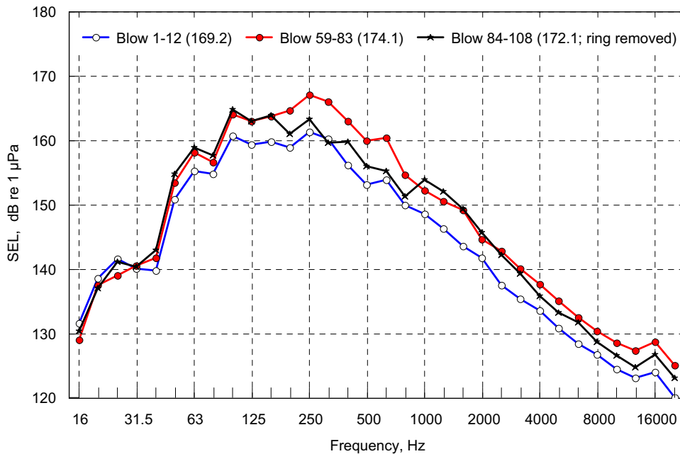
Fig. 3-6. Third octave spectra recorded during different phases of the steel cable experiment. Values in brackets are SEL totals.
