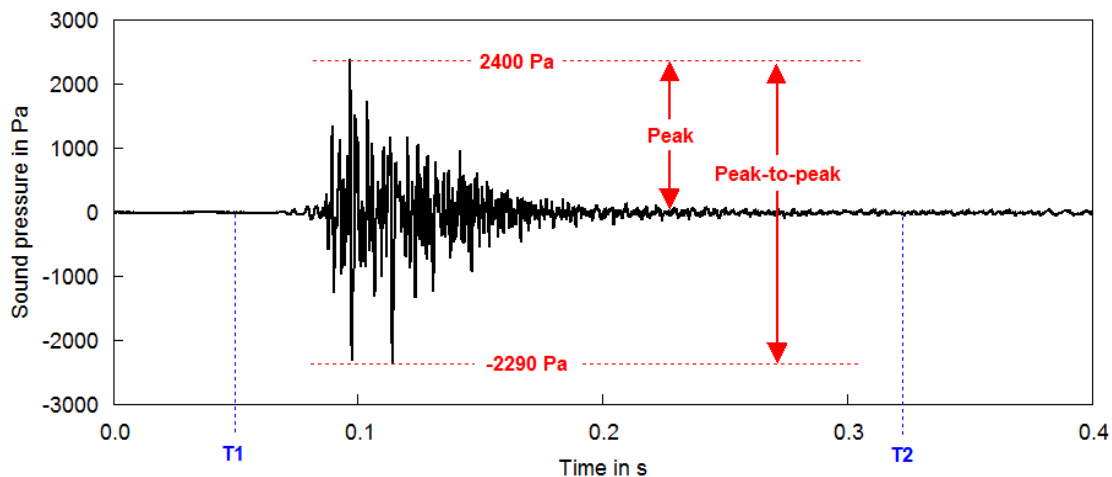
Fig. 2-1. Typical underwater sound pressure impulse of a pile driving stroke in several hundred metres distance. T_1 and T_2 are explained in the definition of the sound exposure level, see equation 2.2. The peak level in this example is 20 \log(2400/10^{-6}) dB = 187.6 dB, whereas the peak-to-peak level is 20 \log((2400+2290)/10^{-6}) dB = 193.4 dB.
