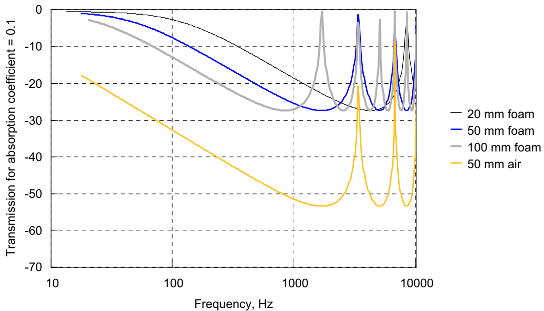
Figure 3-23. As Figure 3-22, but with imperfect sound absorption inside the pile sleeve
