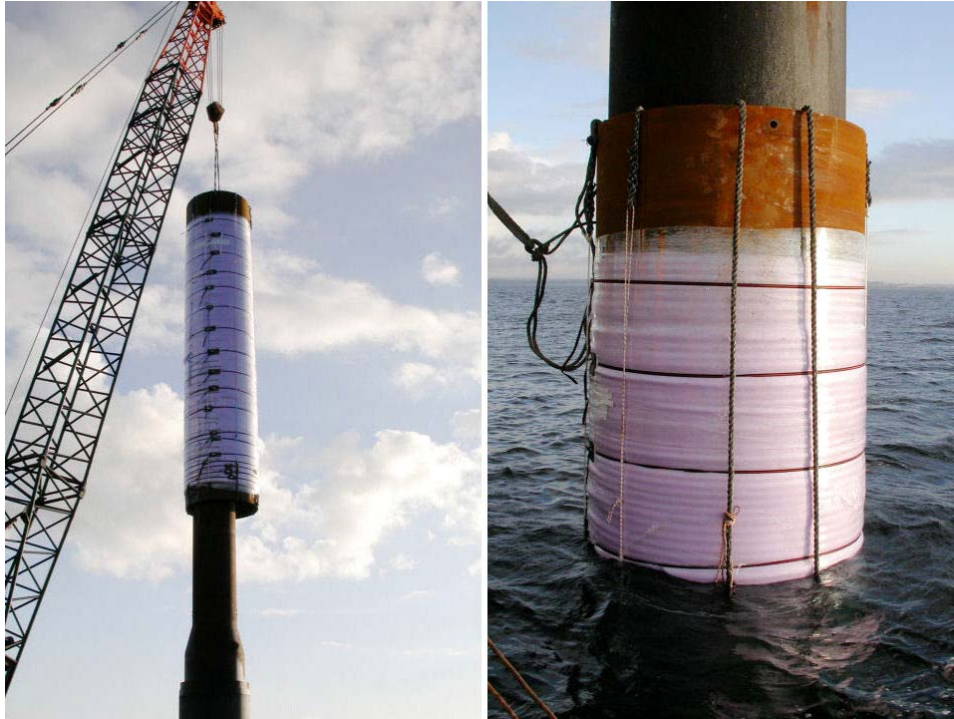
Figure 3-25. Foam-coated steel tube in measurement position (right)
