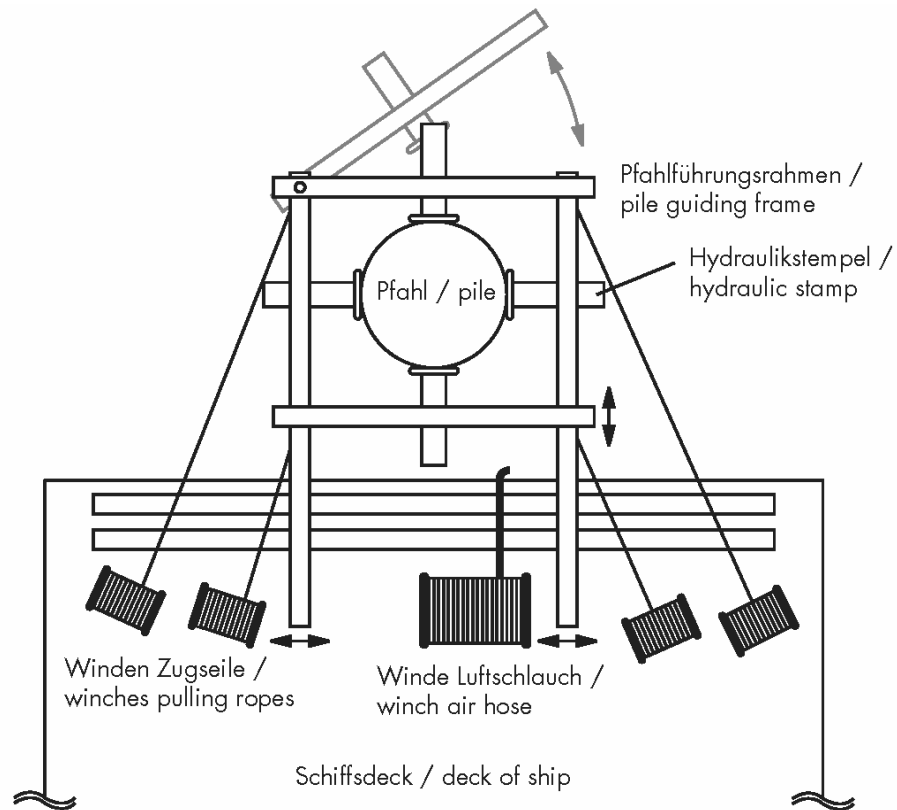
Figure 3-31. Top view: pile guiding frame with winches. Angular guiding frame
