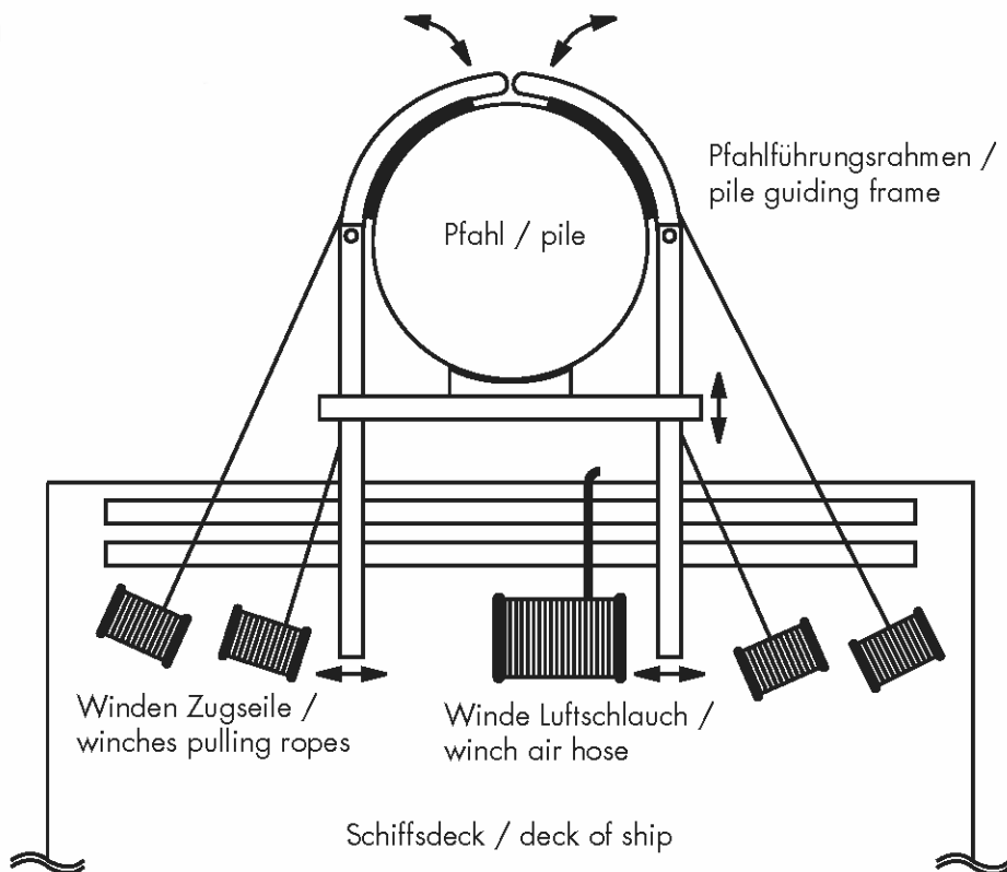
Figure 3-32. Top view: pile guiding frame with winches. Half-round guiding frame
