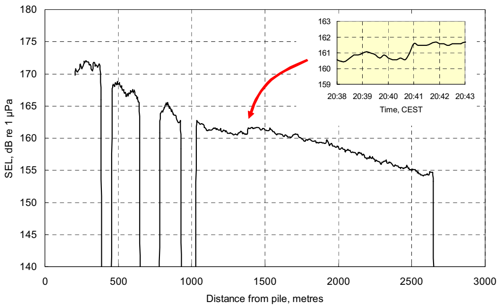
Fig. 2-6. Underwater noise measurement at FINO2 (see Table 2.1) while drifting away from the construction site with a speed of about 0.5 m/s. At 20:41, the blow energy was raised from 250 kJ to 300 kJ, causing a level increase of about 1 dB. The pile driver was an IHC S-500 hydraulic hammer (ISD et al. 2007).
