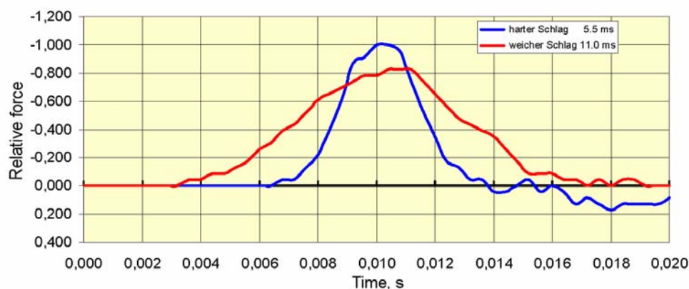
Fig. 3-4. Relative stroke force, measured with sensors (strain gauges) on the pile. Blue curve: "hard" stroke, red curve: "soft stroke" (blow no. 3; see Figure 3-5) with steel cable ring between hammer and pile (Elmer 2007)
