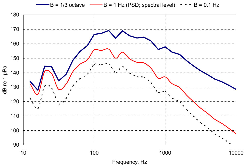
Fig. 2-2. Spectra of sound exposure level (SEL) of a pile stroke, measured with different bandwidths
