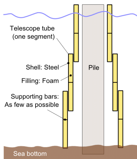
Figure 3-34. Telescopic noise mitigation tube (schematically, not to scale)
