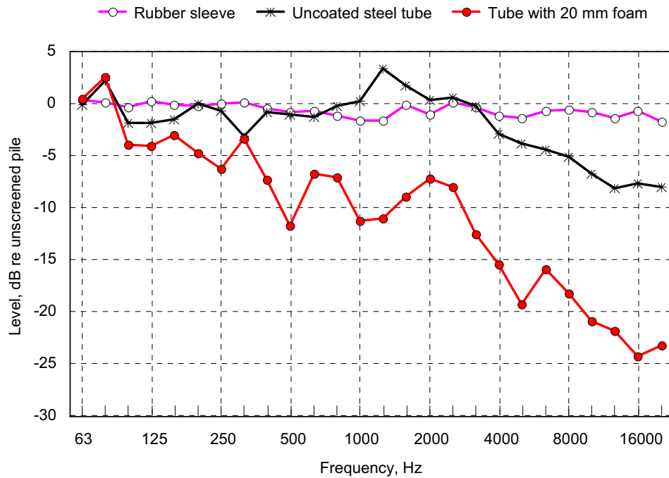
Figure 3-27. Results of the pile sleeve experiments. The foam-coating provides a noise reduction of 10 dB at 1 kHz and 20 dB or more at 10 kHz and above (Schultz-von Glahn et al. 2006).
