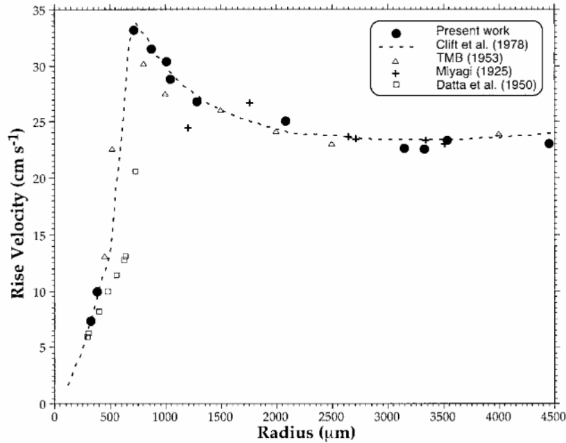
Fig. 3-11. Rise velocity of air bubbles in water at 20°C as a function of bubble size (Leifer et. al 2000)
