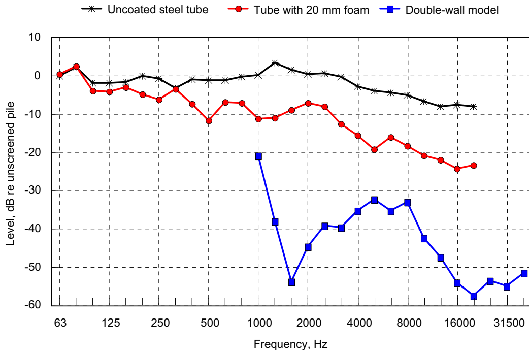
Figure 3-29. Noise reduction measured on the double-wall model. The results with the foam-coated steel tube from Figure 3-27 are shown for comparison. Due to model scale, the measurement was limited to frequencies above 1 kHz (ISD et al. 2007).
