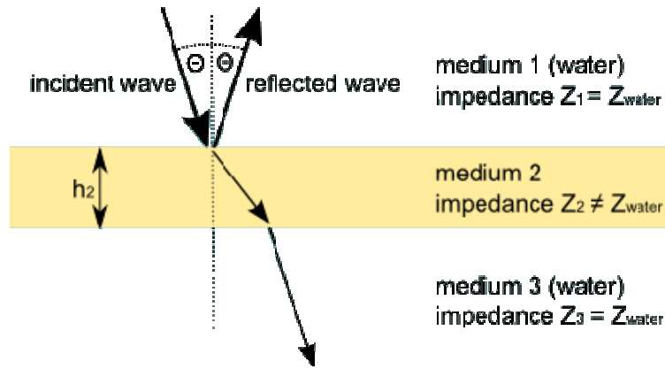
Fig. 3-21. In this configuration, the layer with impedance Z_2 acts as a sound barrier
