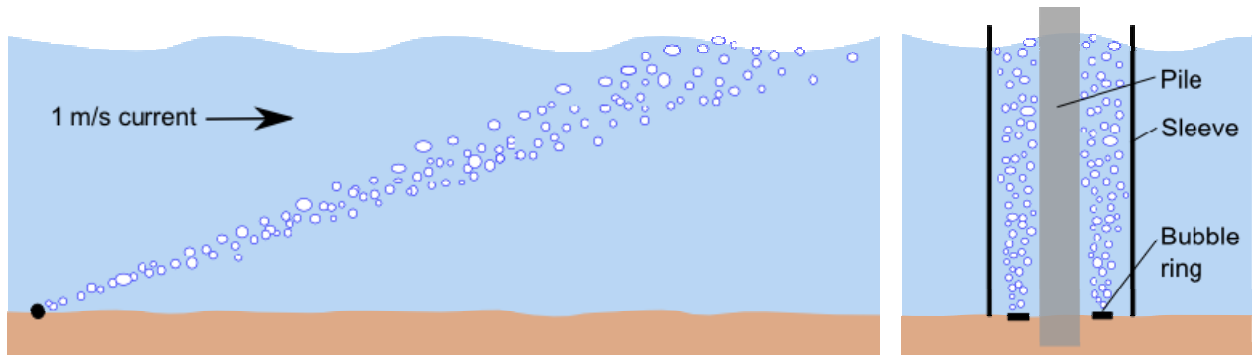
Fig. 3-12. Left: Bubble movement due to current; drift angle approximately to scale for 1 m/s. Right: Confined bubble curtain
