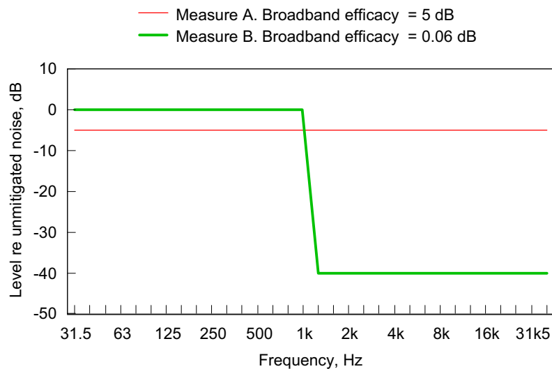
Fig. 3-1. Two hypothetical noise mitigation measures with different sound reduction versus frequency. When applied to pile driver noise, method B yields a poor single-number value though it might be the better one for avoiding disturbance to marine mammals at larger distances from the construction site.
