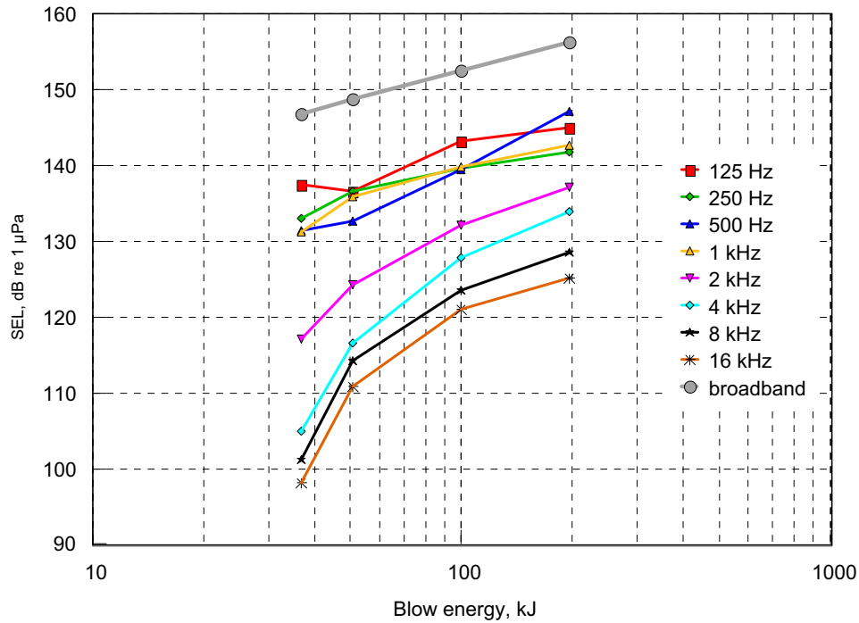
Fig. 2-5. Underwater level as a function of blow energy, produced by a drop hammer (MENCK MHF 10-20) on a 2.2 m pile in 500 m distance. Energies were 37 kJ (minimum setting for this pile driver), 50 kJ, 100 kJ and 200 kJ (Schultz-von Glahn et al. 2006).
