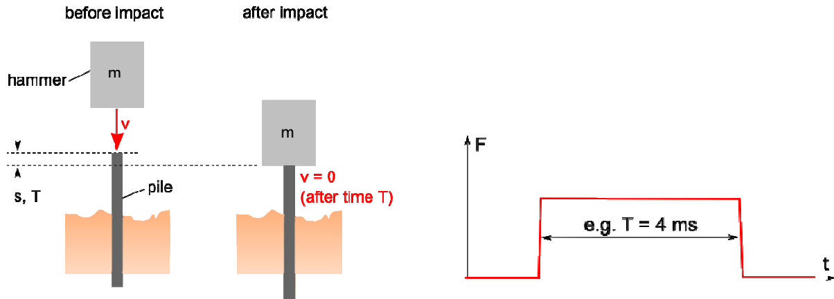
Fig. 3-2. Simplified model of hammering. The hammer hits the pile with velocity v . After the impact, hammer and pile move downwards together a distance s within time T . The velocity is reduced to zero within this time. This means a (negative) acceleration and, because force = mass times acceleration, a force F acting on the pile for a time period T .
