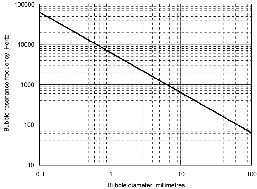
Fig. 3-9. Resonance frequency of an air bubble in water at sea level as a function of diameter
