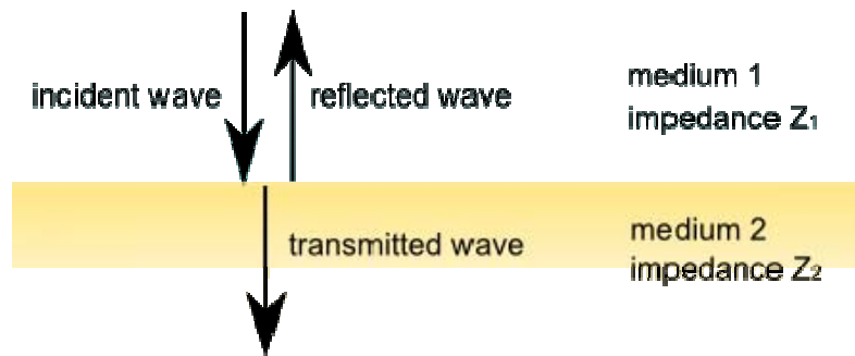
Fig. 3-20. If a sound wave encounters an impedance change from Z_1 to Z_2 , the sound is partly reflected and only part of the sound energy is passed into medium 2.
