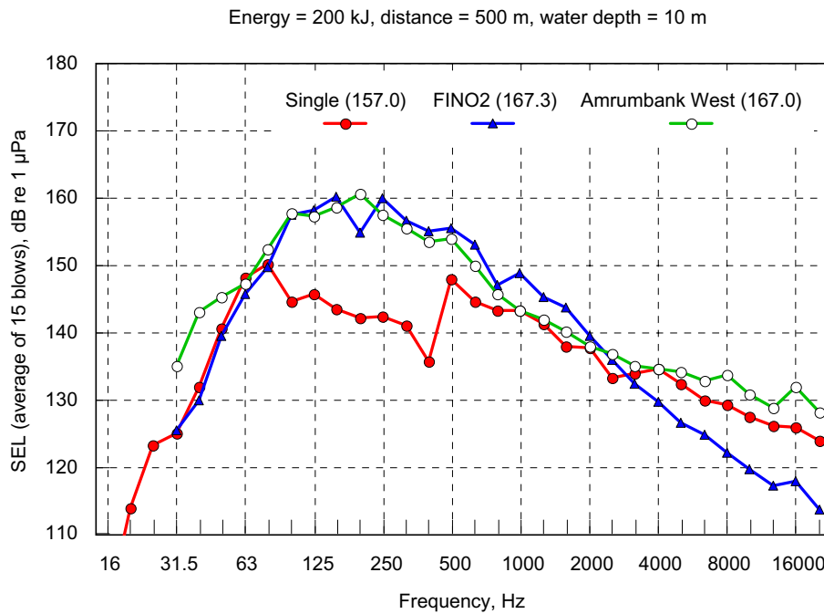
Fig. 3-7. Spectra of pile strokes produced with a single-acting pile driver (drop hammer) and with two double-acting pile drivers. Levels are normalised to equal blow energy, distance and water depth. Values in brackets are SEL totals.
