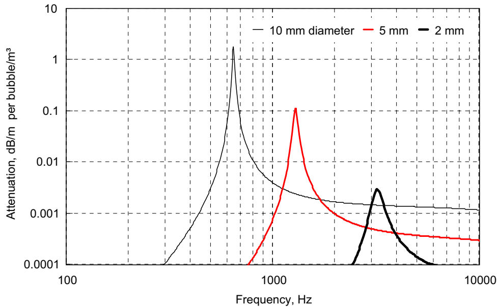
Fig. 3-10. Sound attenuation after equation 3.1 for various bubble sizes
