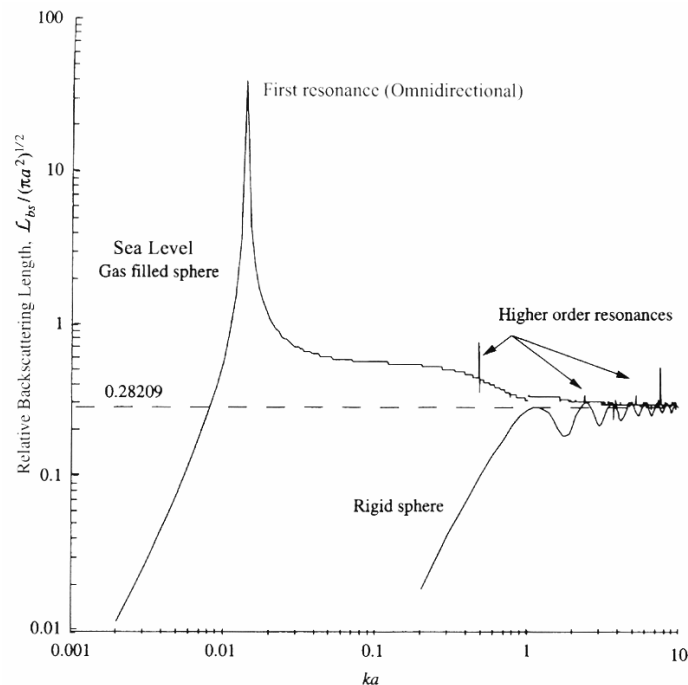
Fig. 3-8. Backscattering length of a gas bubble in water compared to that of a rigid sphere (Medwin 2005, fig. 6.12)
