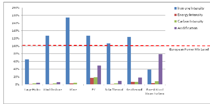
Figure 17 Energy and CO 2 intensities compared with the European Power Mix level [20].
