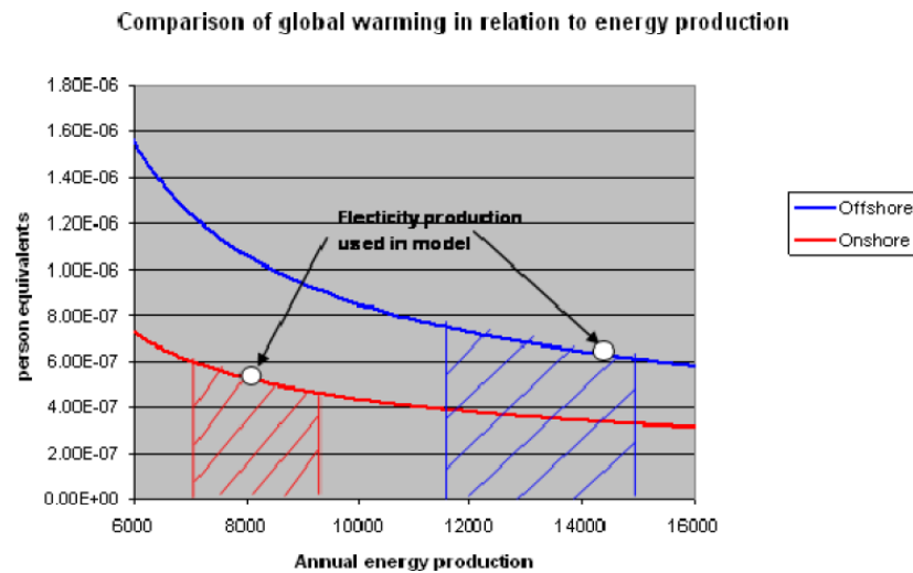
Figure 22 Comparison of global warming impact of V90 wind turbine in relation to energy production onshore and offshore.
