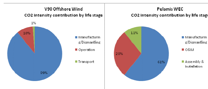
Figure 18 Carbon distribution for offshore wind and wave converter Pelamis ([3], [5], [20]).
