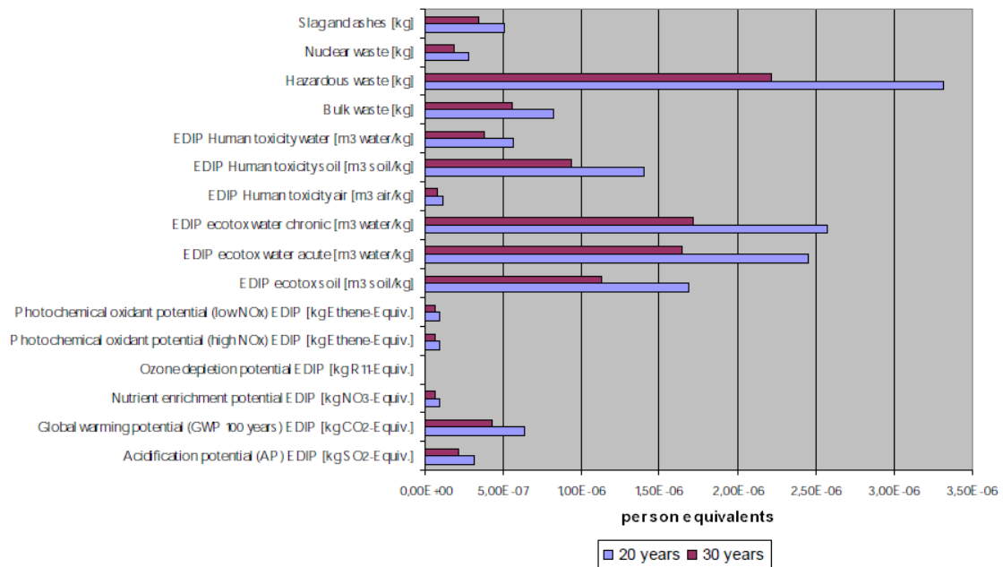
Figure 23 Lifetime influence on environmental effects.
