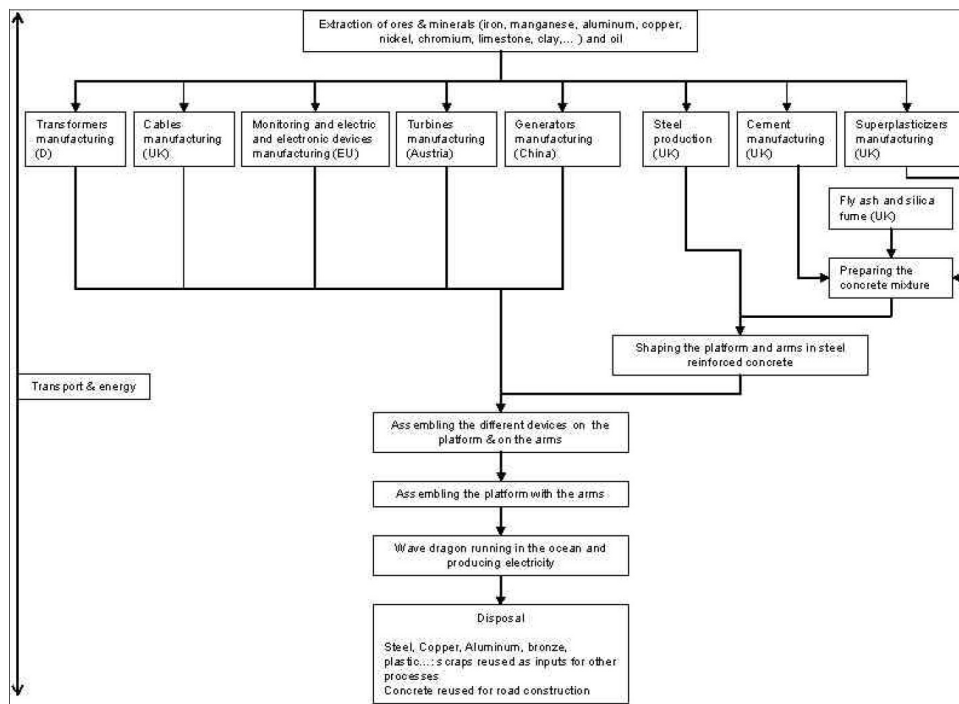
Figure 6 Flow chart of the life cycle of Wave Dragon [9].
