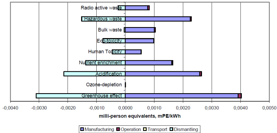
Figure 20 Environmental impacts of 1kWh from Horns Rev offshore wind farm divided into stages [4]
