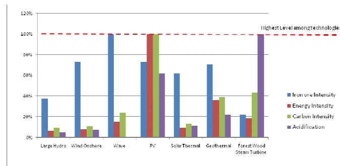
Figure 16 Energy and CO 2 intensities compared with the worst performance [20].
