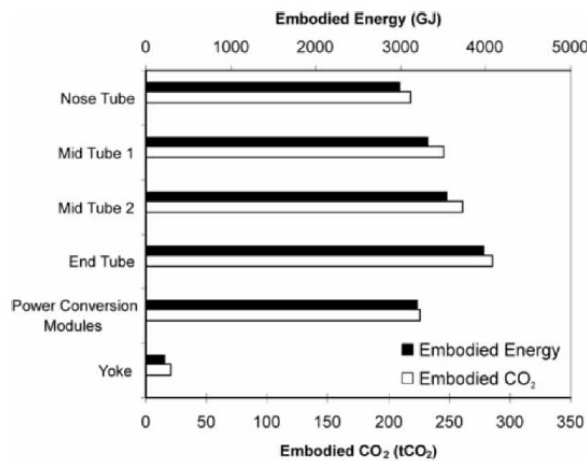
Figure 21 Structural embodied energy and CO 2 on Pelamis P1 device [3].
